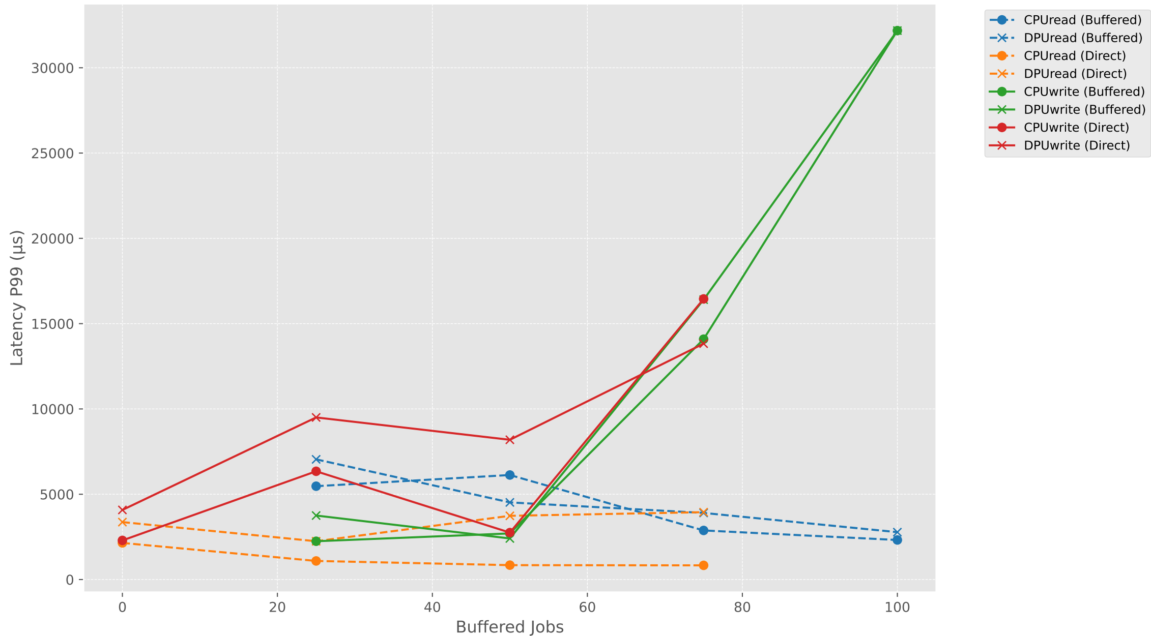
Latency P99 vs Buffered Jobs (mixed) - SEQ (CPU vs DPU)
